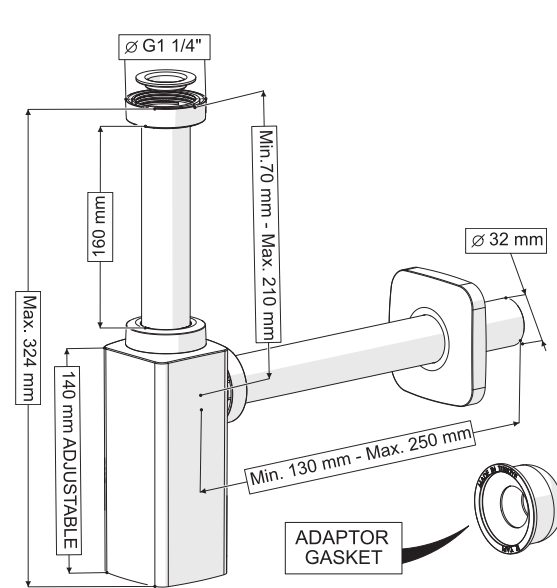
250 mm QUAD SIPHON WITHOUT HOLE ELIXIR POP-UP
