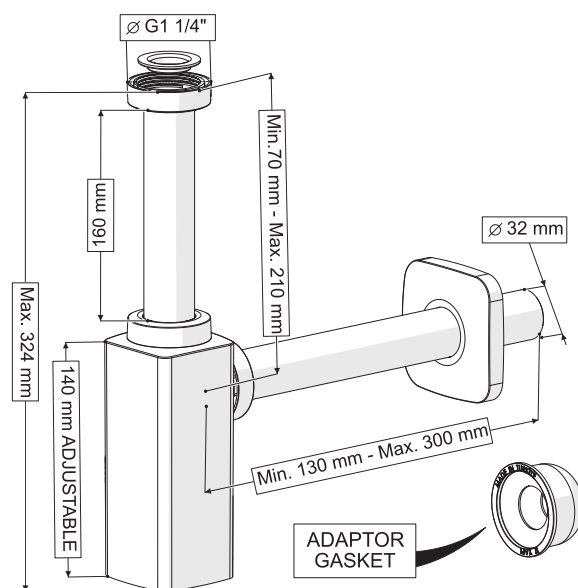
300 mm QUAD SIPHON WITHOUT HOLE ELIXIR POP-UP
