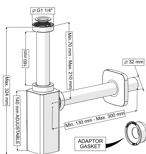
300 mm QUAD SIPHON WITHOUT HOLE ELIXIR POP-UP
