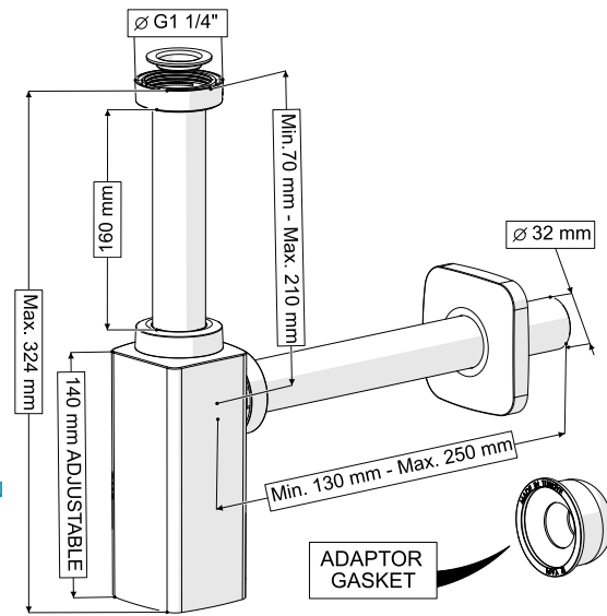
250 mm QUAD SIPHON WITHOUT HOLE ELIXIR POP-UP
