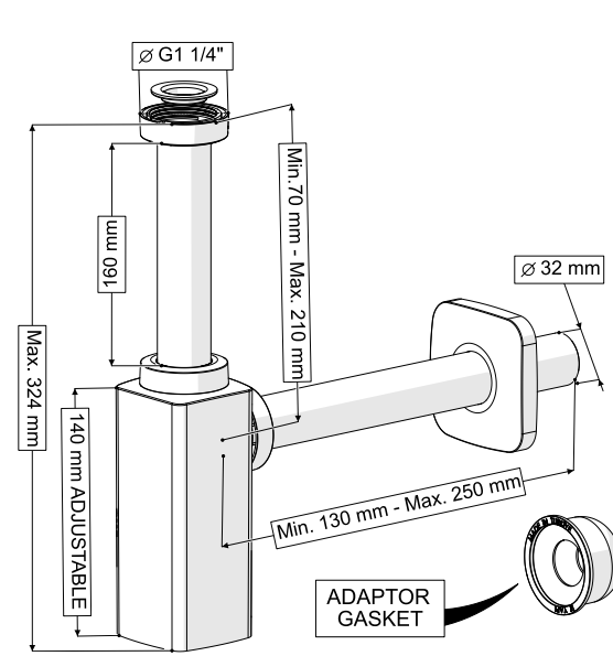
250 mm QUAD SIPHON WITHOUT HOLE ELIXIR POP-UP
