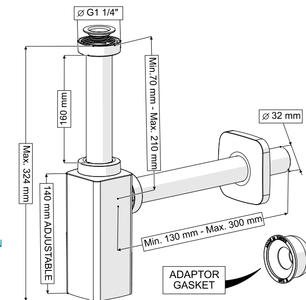
300 mm QUAD SIPHON WITHOUT HOLE ELIXIR POP-UP
