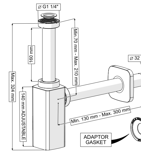
300 mm QUAD SIPHON WITHOUT HOLE ELIXIR POP-UP
